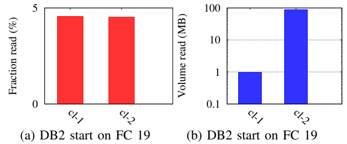
Fig. 7. Fraction and volumes of base image reads while starting DB2 10 on FC 19.
