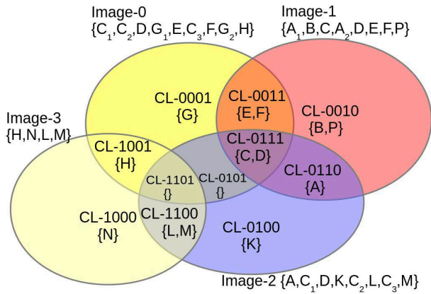
Fig. 1. Illustration of content clusters for four VM images. Upper case letters denote non-identical blocks. Identical blocks can appear more than once in the same image and are differentiated by the use of subscript
