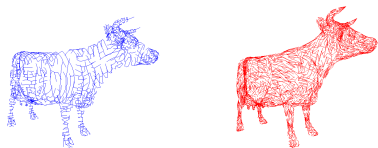
Fig. 4. We compute condition numbers for several 3D surface meshes, comparing tree preconditioning and Jacobi-tree preconditioning. Meshes are endowed with both minimum (blue) and maximum (red) spanning trees (weights correspond to Euclidean edge length).
