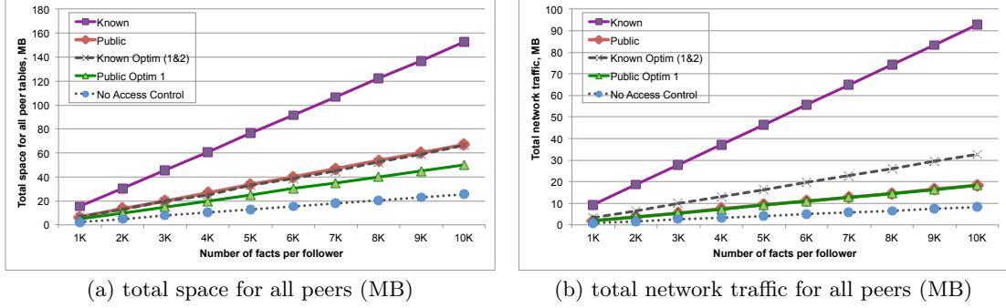
Figure 10: Space overhead of access control, for MAF-JoU (10/2/1).
