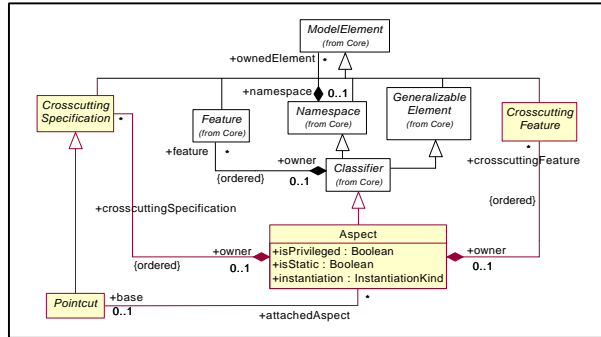
Figure 1. Abstract Syntax of Aspect
