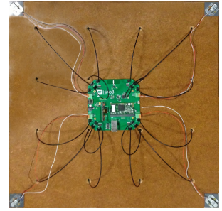
(b) The underneath of the load-sensing tiles used, showing the load sensors located in the corners.
