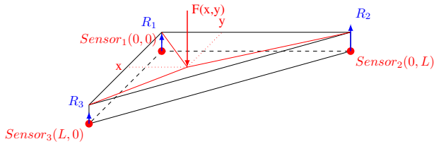
Fig. 1: Load distribution on an isostatic tile
