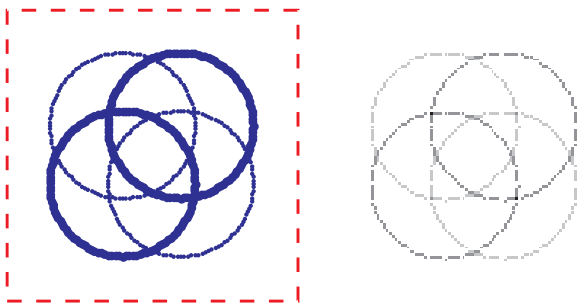
(a) An example with four crossed circles, two of which are 2 times heavier than the other ones. Object thickness represents weight here, and is otherwise not representative.
