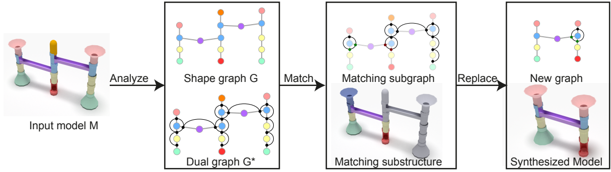
Figure 2: Pipeline: The input is one or more segmented 3D models, with parts of related functionality labeled consistently as shown in the shape(dual) graph. We propose a polynomial time algorithm to enumerate all the matching subgraphs that could be replaced at alternative locations in the model to create plausible shape variations (see Figure 4 and Section 4.4 for details).
