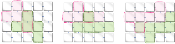
Figure 6: Even simple graphs (here: regular grid of identical parts) can have an exponential number of matching cuts. However, due to symmetry, all but an \mathcal{O}(k \cdot n^2) -sized subset have the same effect.
