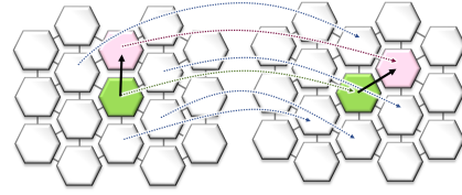
Figure 7: A partial graph symmetry is fixed by one node and one edge assignment.
