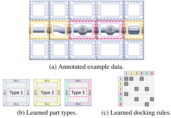
Figure 3: A simple example for learning docking rules. (a) The original input data is annotated with parts and docking sites. (b) This yields parts of different types and (c) rules for connecting them, visualized as a compatibility matrix.
