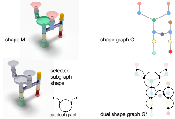
Figure 4: From a shape M with annotated part types (indicated by color) we construct a shape graph G where each part becomes a node and each part-connection an edge. The dual graph G^* encodes how a set of parts can be removed to extract a subgraph. In this example (bottom-left), the cut is formed by removing two nodes from the dual graph G^* .
