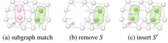
Figure 5: Graph operations modify existing shape graphs by replacing matching subgraphs iteratively.
