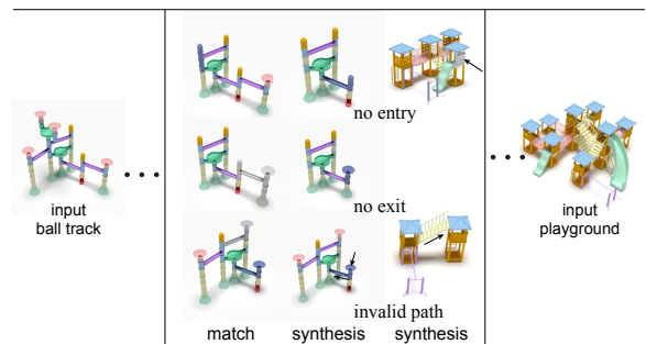
Figure 12: Various synthesis results marked as invalid due to violation of global constraints (e.g., no entry, no exit, or no connections between entry-exit).
