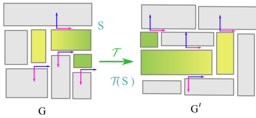
Figure 10: Non uniform interpolation weighting across parts and inside parts create non-rigid transformations.
