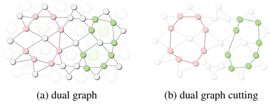
Figure 8: Manifold-like data is created by ordering docking sites (see Figure 5). In a dual graph, matching cuts is performed by node propagation.
