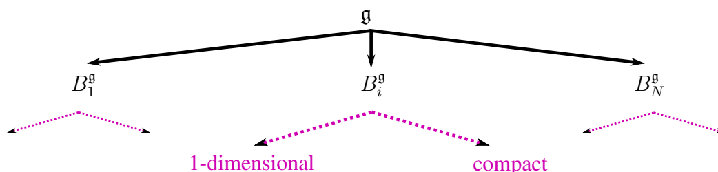
Figure 3. Structure of a Lie algebra with bi-invariant metrics.
