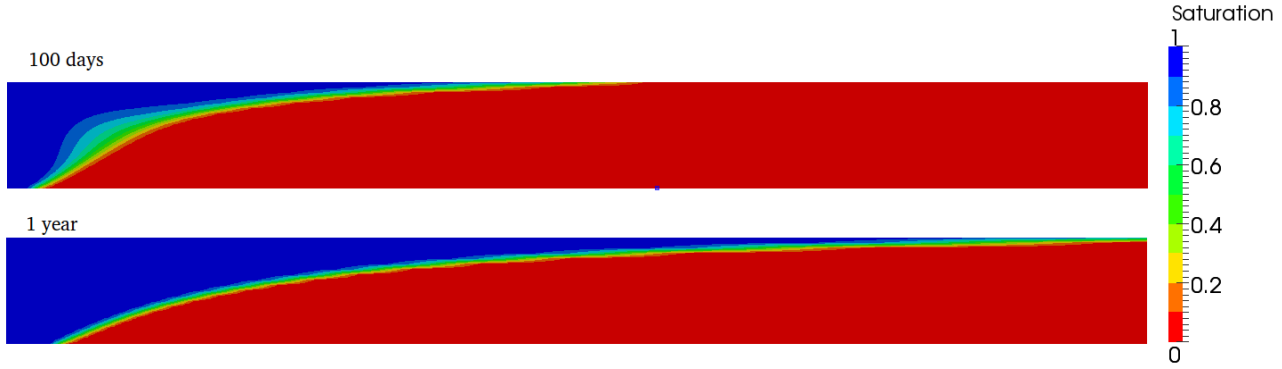
FIGURE 3. Liquid saturation S_l after 100 days and 1 year of \text{CO}_2 injection. Only the 1.1 km closest to the injection is presented.
