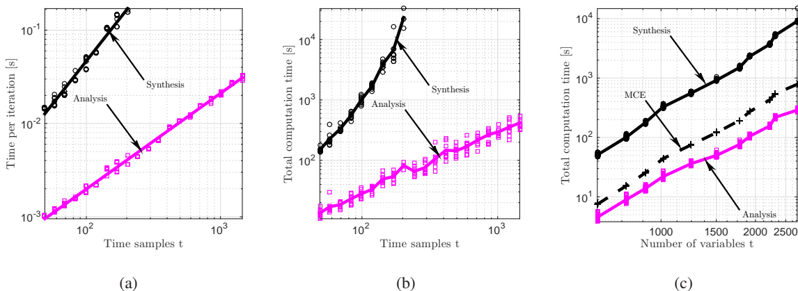
Figure 1. Computation time relative to the problem size. (a) Time per LSMR iteration vs t (wave equation). (b) Total computation time vs t (wave equation). (c) Total computation time vs n (Poisson's equation).
