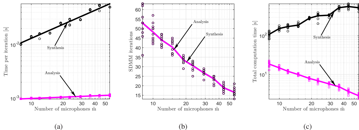
Figure 2. Computational cost vs number of microphones \tilde{m} . (a) Time per LSMR iteration. (b) Number of SDMM iterations. (c) Total computation time.
