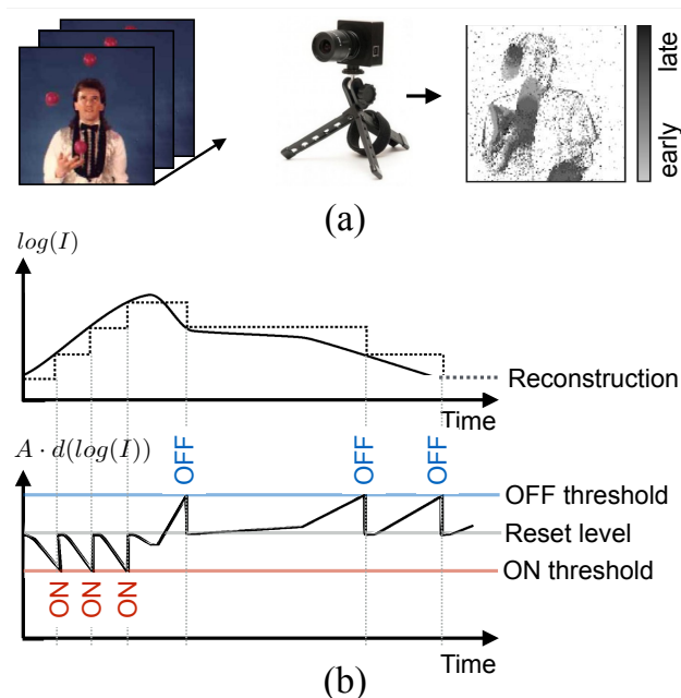
Figure 5: How DVS sensor generate spikes. (a) Example of a video with fast motions (a juggling scene). DVS camera and DVS output: Events are rendered using a grayscale colormap corresponding to events that were integrated over a brief time window (black = young, gray = old, white = no events). (b) DVS principle: Positive and negative changes are generated depending on the variations of \log(I) which are indicated as ON and OFF events along temporal axis (adapted from [184], with permissions).
