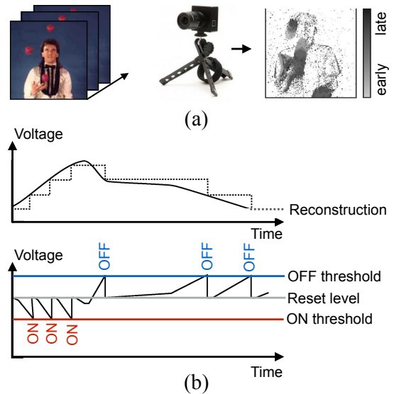
Figure 5: How DVS sensor generate spikes. (a) Example of DVS output in response to a juggling scene (down). Events are rendered using a grayscale colormap corresponding to events times (black = young, gray = old, white = no events). (b) DVS principle: Positive and negative events are generated depending on the variations of \log(I) which are indicated as on and off events along temporal axis. (Adapted from [177], with permissions.)
