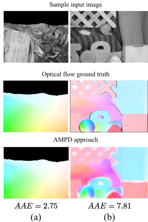
Figure 8: Example of results obtained with the approach called Adaptive Motion Pooling and Diffusion (AMPD) for two classical videos: (a) Yosemite and (b) Rubberwhale from Middlebury dataset. AMPD is an extension of the feedforward spatio-temporal filter based model by Heeger and Simoncelli (HS) [292] model incorporating contrast adaptation, adaptive afferent pooling and MT diffusion dependent upon the local 2D image structure.
