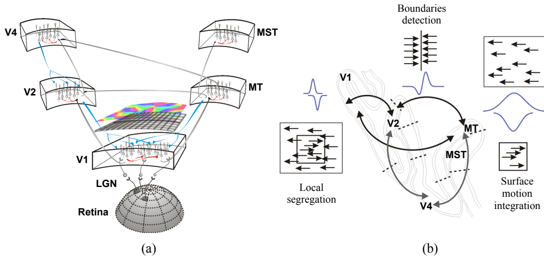
Figure 3: (a) A schematic view of the early visual stages with their different connectivity patterns: feedforward (grey), feedback (blue) and lateral (red). (b) A sketch of moving surface segmentation and its potential implementation in the primate visual cortex. The key processing elements are illustrated as computational problems (e.g. local segregation, surface cues, motion boundaries, motion integration) and corresponding receptive field structures. These receptive fields are highly adaptive and reconfigurable, thanks to the dense interconnections between the different stages/areas
