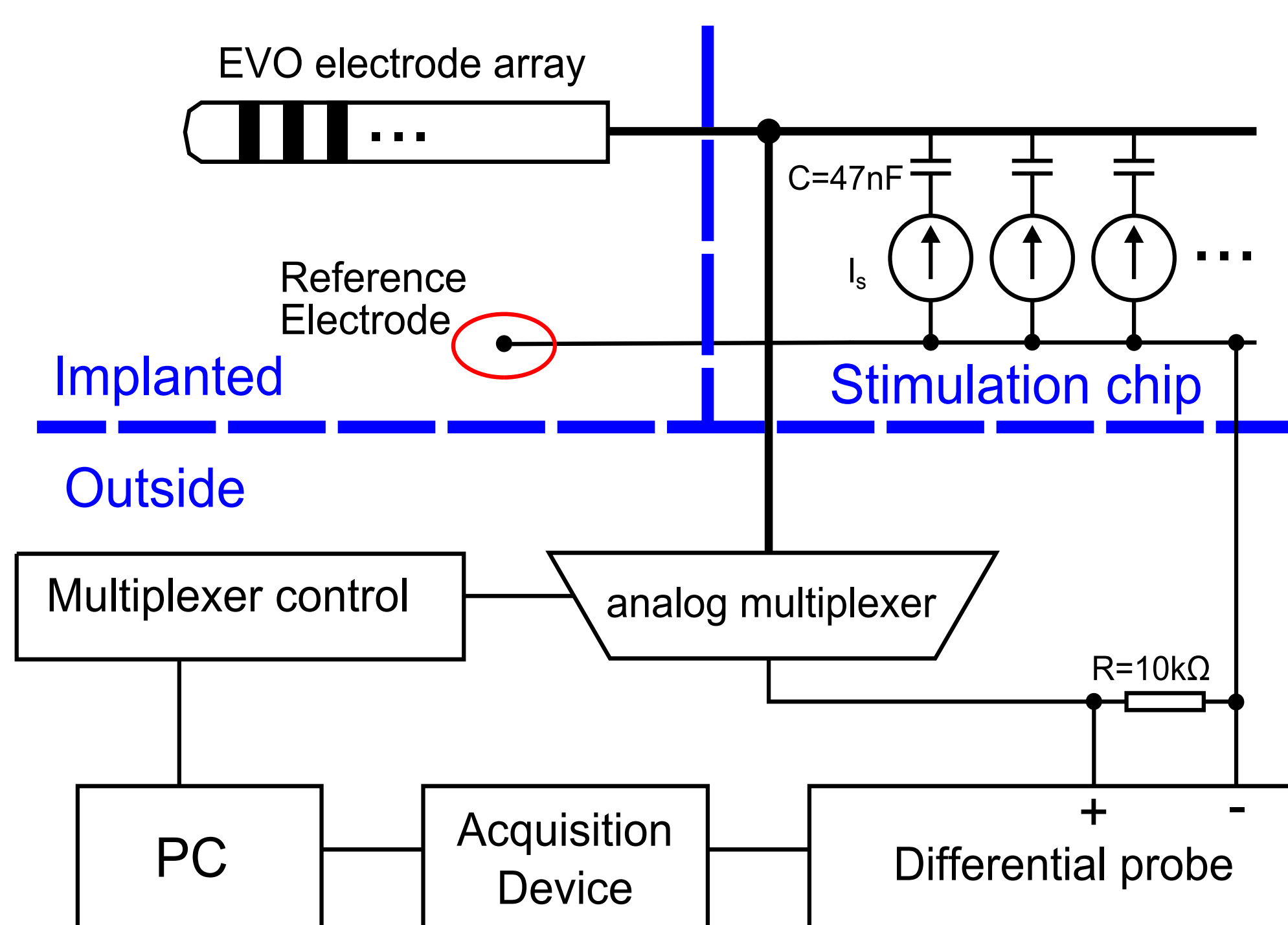
Figure 1. Diagram of the stimulation-recording system[2]
