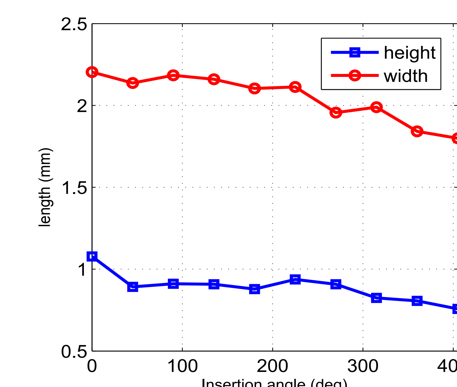
Figure 7. Width and height of the scala vestibuli measured from micro-CT scan
