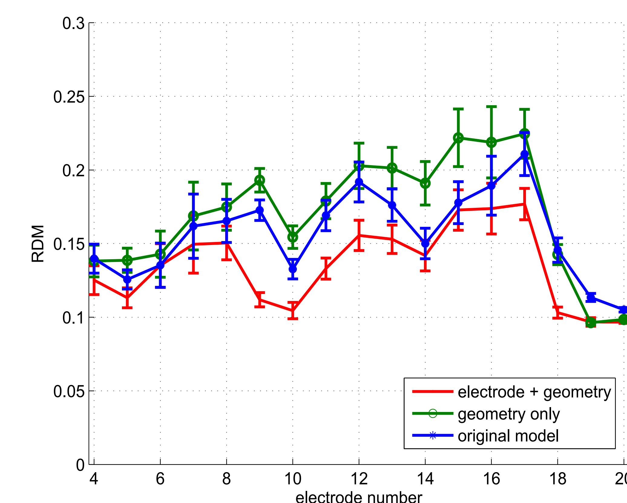
Figure 5. Simulation error under bipolar stimulation mode
