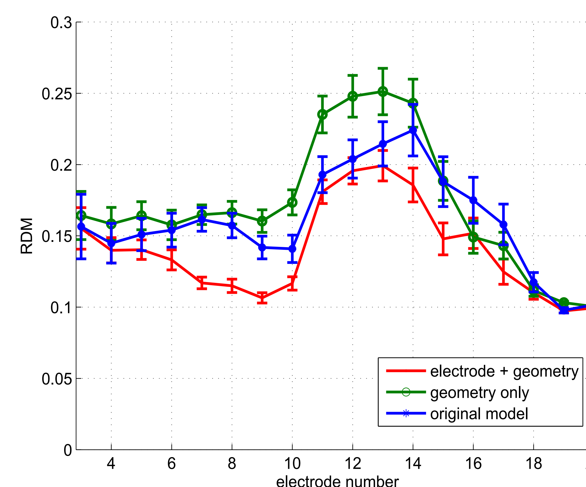
Figure 6. Simulation error under monopolar stimulation mode
