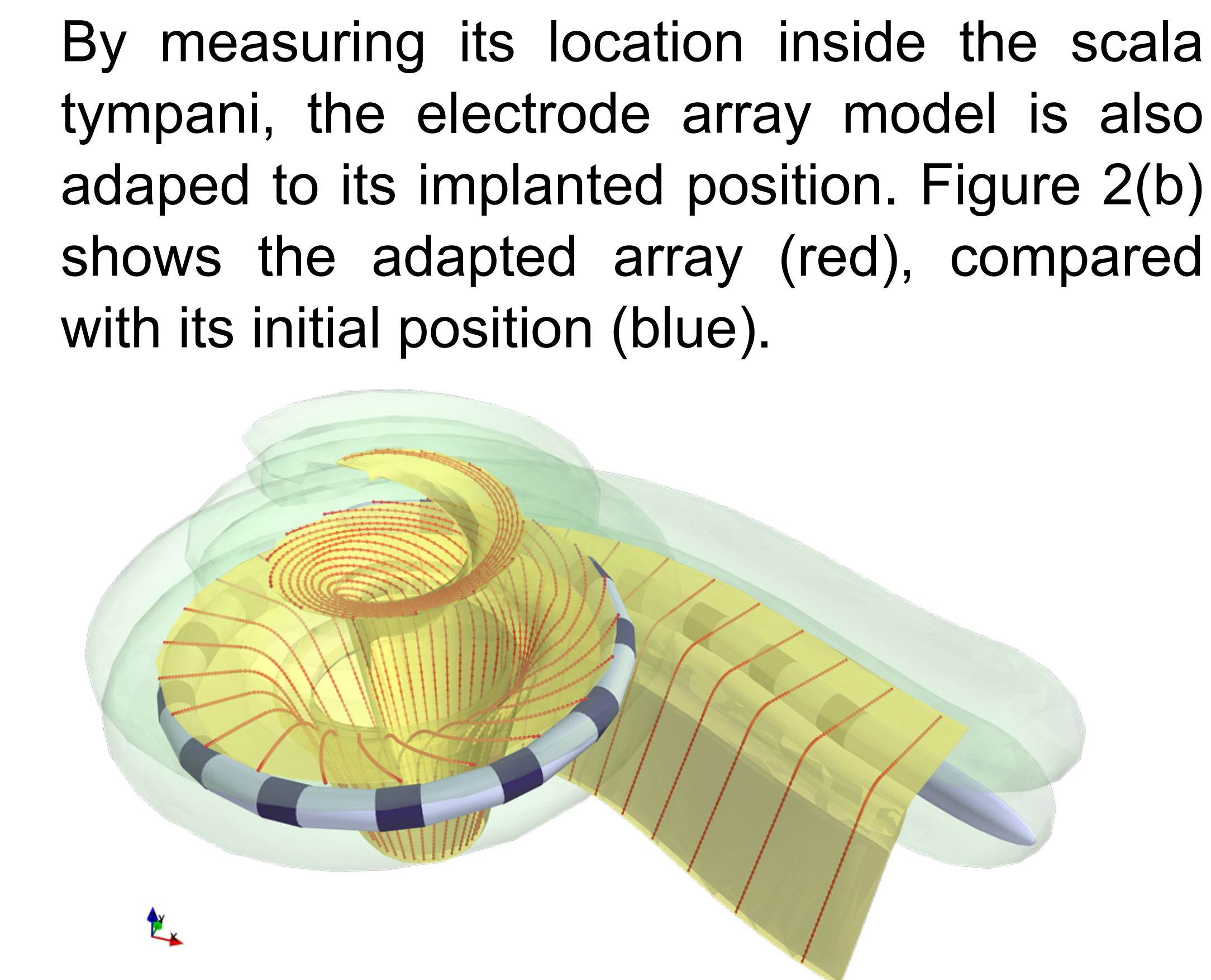
Figure 3. Snapshot of the parametric cochlear model
