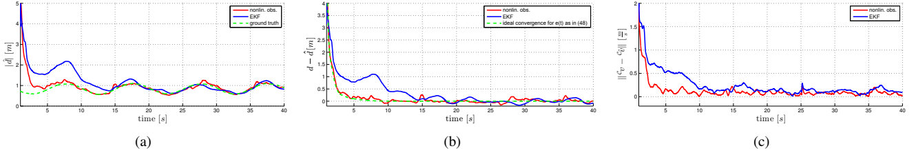
Fig. 12: Experimental results — Results from flying along an inclined circular trajectory, thus involving a time-varying d(t) . (a) Estimated \dot{d}(t) for the nonlinear observer and EKF, (b) Estimation error d(t) - \hat{d}(t) and ideal convergence behavior (48) for the nonlinear observer, and (c) norm of the velocity estimation error against the ground truth. Note, again, the very good performance of the nonlinear observer in recovering d(t) and v(t) despite the more challenging UAV motion (as well as, again, the almost perfect match between the actual and ideal transient response of the estimation error)
