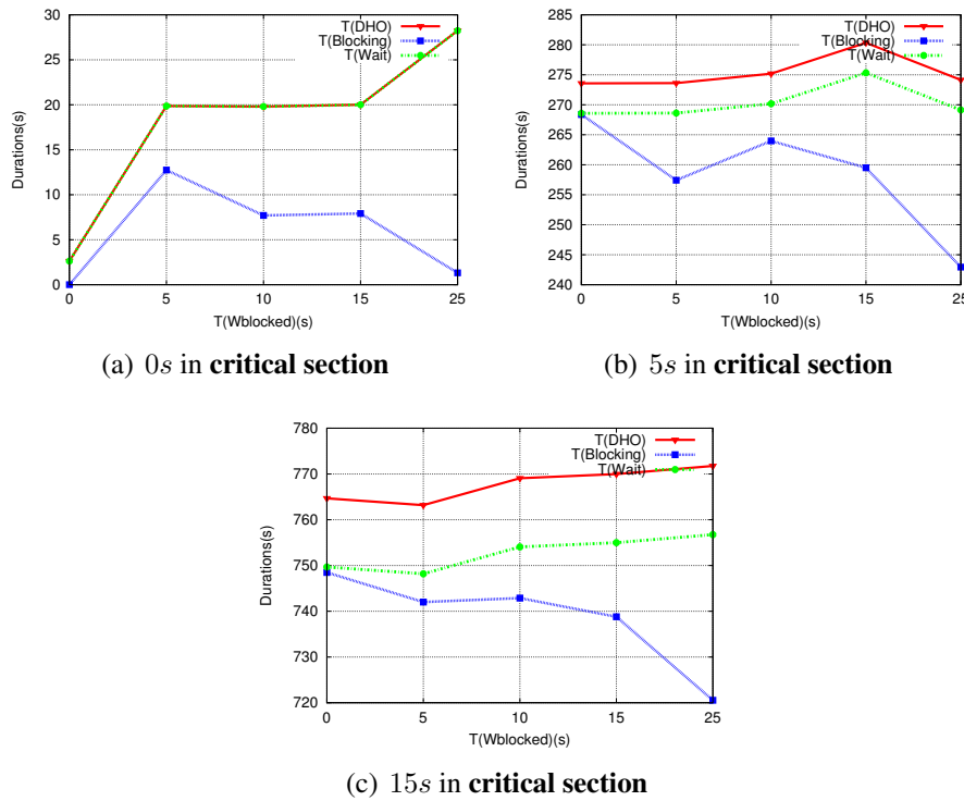
Figure 7: Average duration of \overline{T_{\text{DHO}}} , \overline{T_{\text{Wait}}} and \overline{T_{\text{Blocking}}} by varying T_{\text{Wblocked}} .
