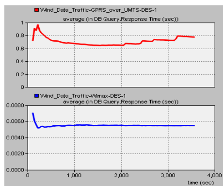
Figure 11. Average response time in Database Query
