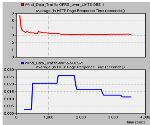
Figure 13. Average Page response time in HTTP service
