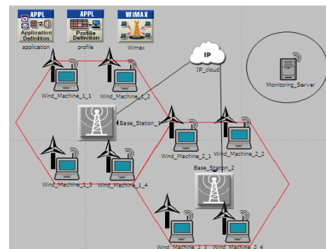
Figure 10. Wi-Max wind park monitoring OPNET scenario
