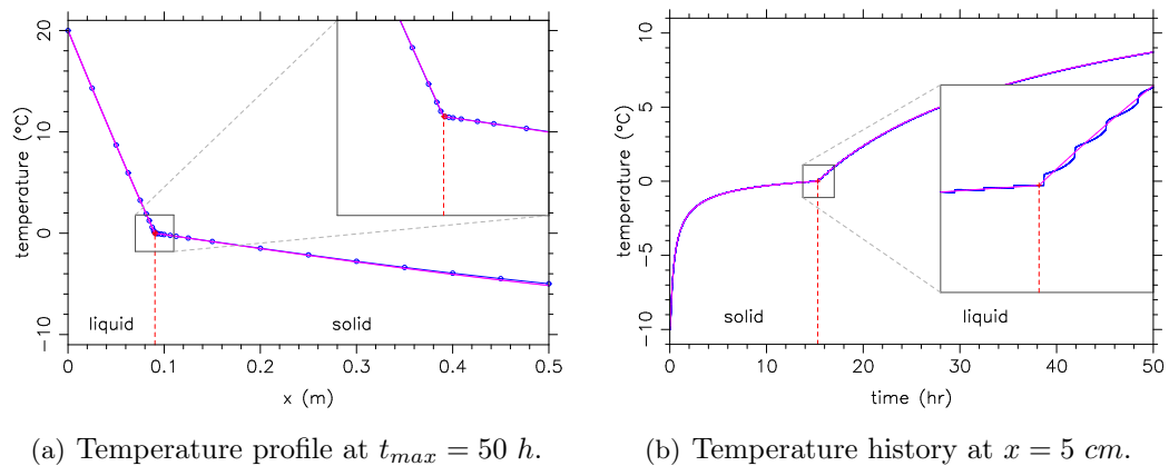
Figure 5: Rolling mesh, N_{basic} = 40 , dt = 2.72E - 01 \text{ s} , Number of subdivisions: 6. Analytical (red) and numerical (blue) solutions.
