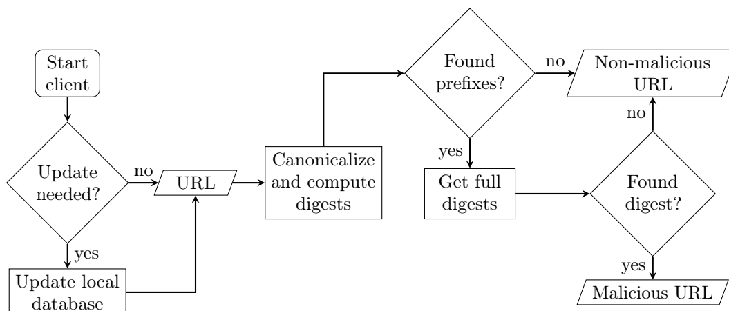
Figure 2: GOOGLE Safe Browsing API: Client's behavior flow chart.
