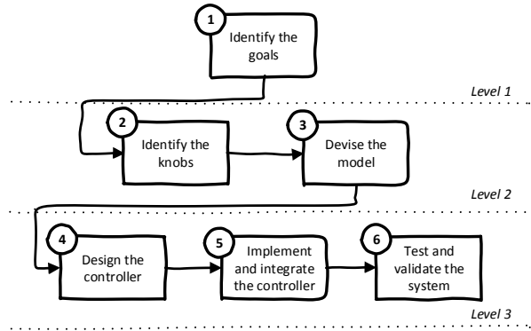
Fig. 3: Steps in the design and development of a control-based mechanism for self-adaptive systems. The different levels group steps into activities with tighter coupling.
