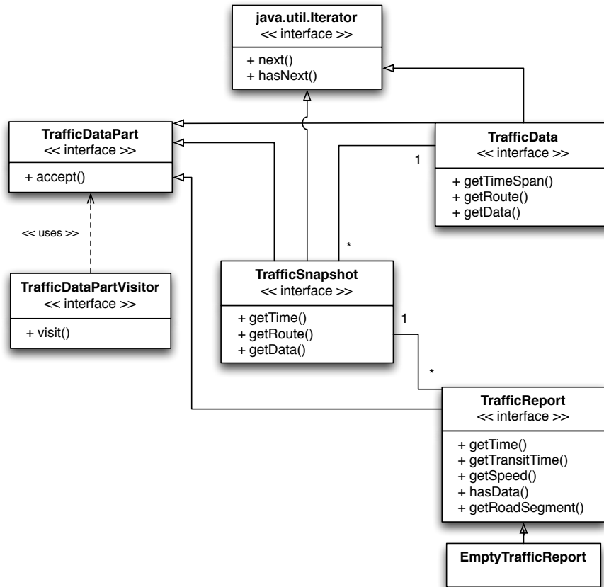
Figure 4.7: Overview class diagram of traffic data package. Not all available methods are listed; arguments and return types were omitted.
