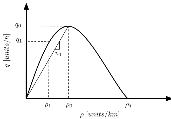
(c) flow vs. density
