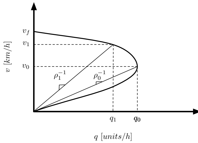
(b) speed vs. flow
