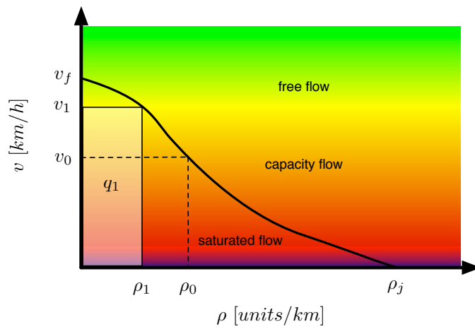
(a) speed vs. density
