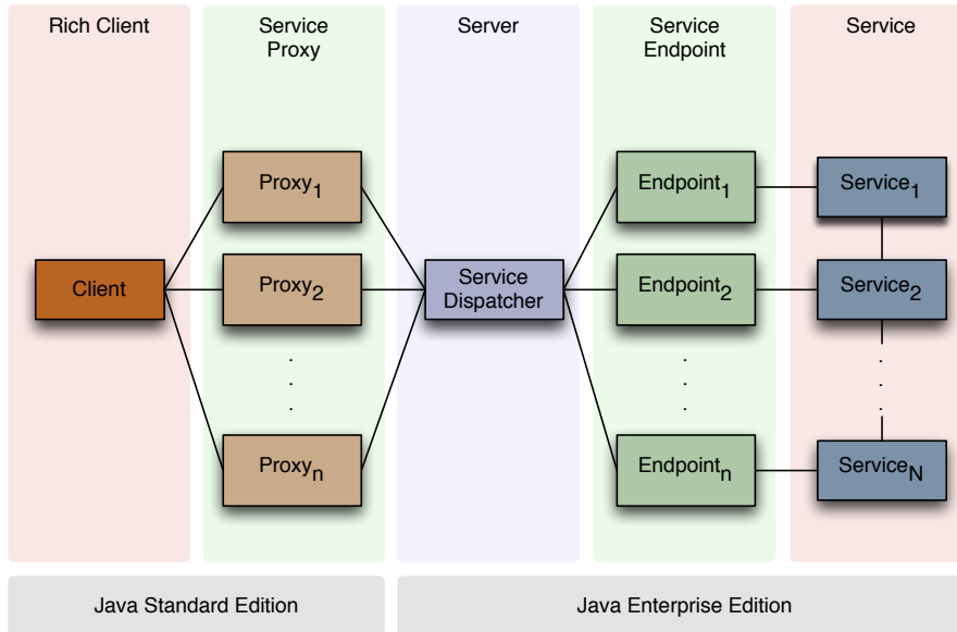
Figure 4.2: Client-server communication
