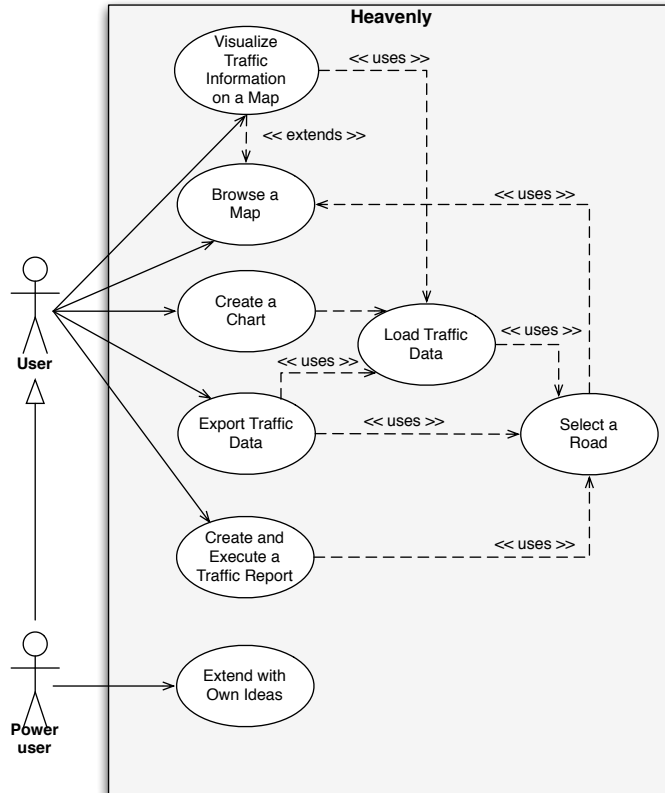
Figure 3.3: Use cases
