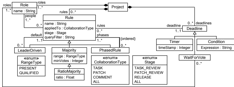
Fig. 3. Abstract syntax metamodel of our DSL to represent governance rules.
