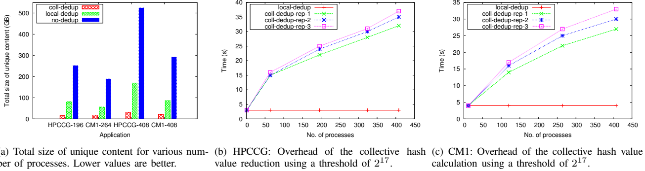
Fig. 3. Effectiveness of deduplication: size of unique content and scalability of collective hash value reduction overhead.
