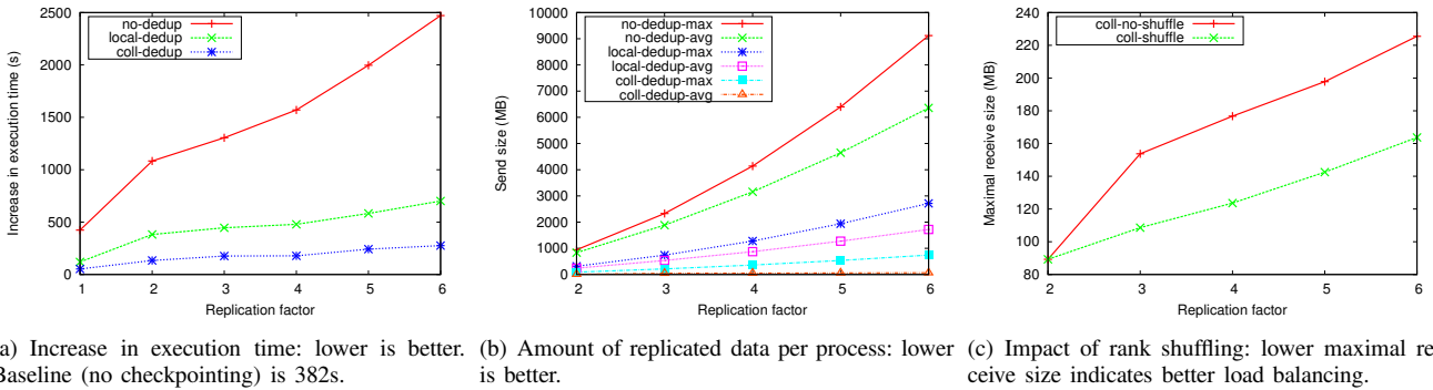
Fig. 5. CM1: scalability results for increasing number of replicas. Problem size is 408 processes (corresponding to 34 nodes).
