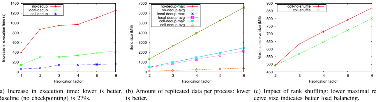
Fig. 4. HPCCG: scalability results for increasing number of replicas. Problem size is 408 processes (corresponding to 34 nodes).
