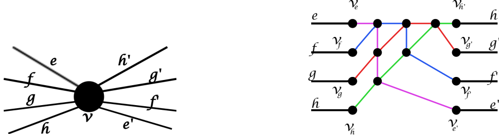
(a) A vertex of degree 8 and allowed transitions A(v) = \{\{e, e'\}, \{f, f'\}, \{g, g'\}, \{h, h'\}\} (edges are ordered as in the planar embedding of G )
