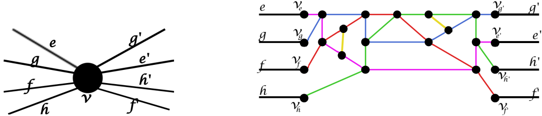
(a) A vertex of degree 8 and allowed transitions A(v) = \{\{e, e'\}, \{e, f'\}, \{f, f'\}, \{f, e'\}, \{g, g'\}, \{g, h'\}, \{h, h'\}, \{h, g'\}\} (edges are ordered as in the planar embedding of G ) (b) Gadget D_v : the paths P_{ee'} , P_{ff'} , P_{gg'} , and P_{hh'} are respectively the pink, red, blue and green paths. transitions around vertices v_i , transitions of the paths P_{ee'} , P_{ff'} , P_{gg'} , and P_{hh'} , and transitions containing the yellow edge are allowed
