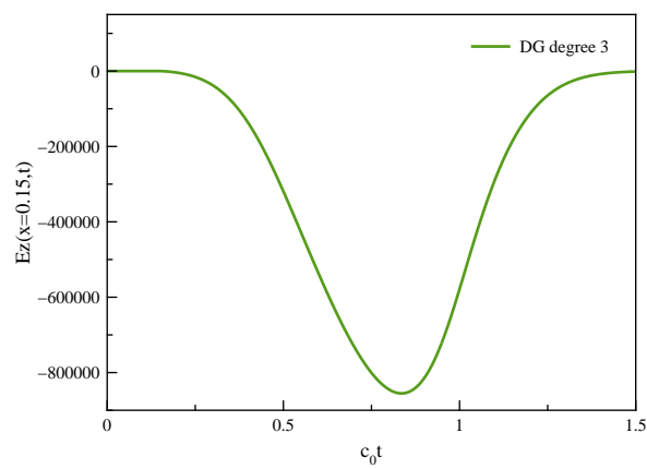
Figure 28: Radiating dipole: medium=air, f = 0.1 GHz : E_z(x = 0.15, t) .
