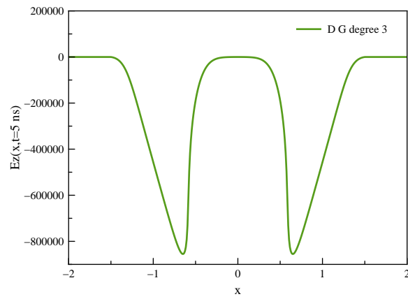
Figure 27: Radiating dipole: medium is air, f = 0.1 GHz : E_z(x, t = 5) .
