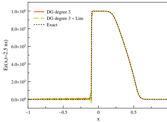
Figure 10: DG method with with Bernsetin polynomial of degree 3, and with limited polynomials.
