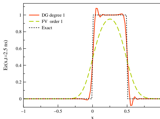
Figure 1: First order FV and DG- \mathbb{P}_1 methods.
