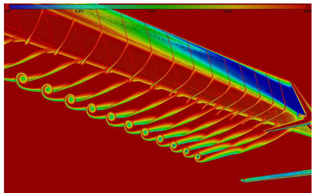
Figure 33. Transonic WBT configuration: velocity isovalues.
