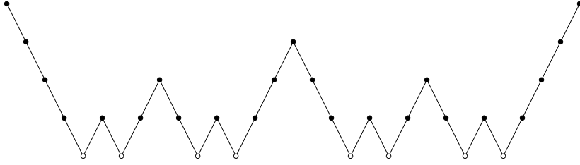
Figure 7. A five-grid method: W-cycle ( \bullet : 1 smoothing SGS iteration, \circ : Several SGS iterations)
