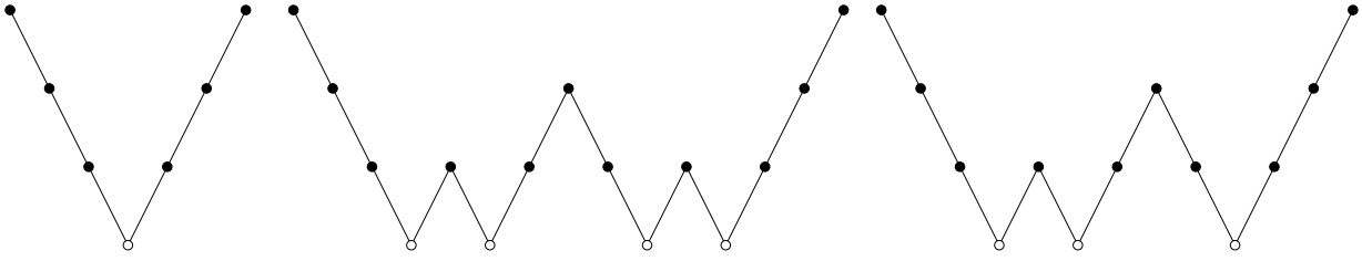
Figure 6. Four-grid methods : V-cycle, W-cycle and F-cycle ( \bullet : 1 smoothing SGS iteration, \circ : Several SGS iterations)
