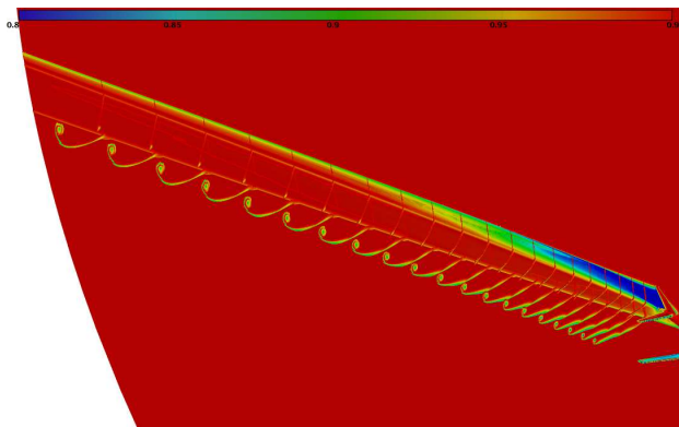
Figure 33. Transonic WBT configuration: velocity isovalues.
