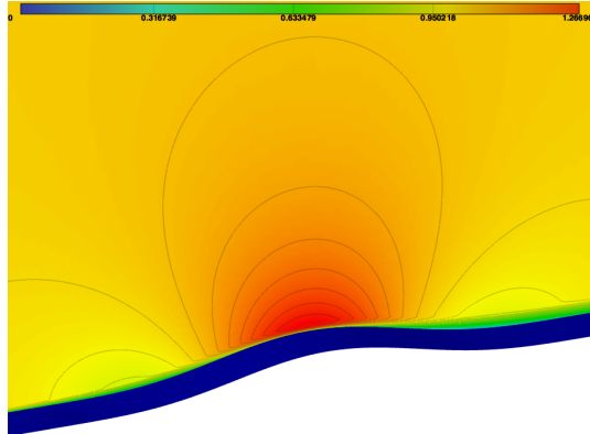
Figure 1. Speed isolines around the bump
