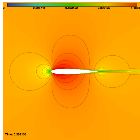
Figure 4. NACA0012: Speed isolines ( \alpha = 0 ).
