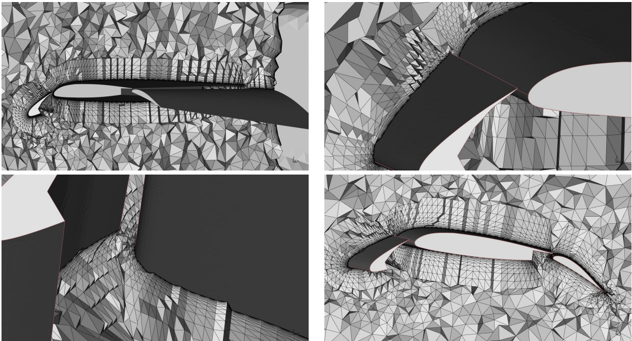
Figure 8. Boundary layer mesh generation around a high lift geometry.
