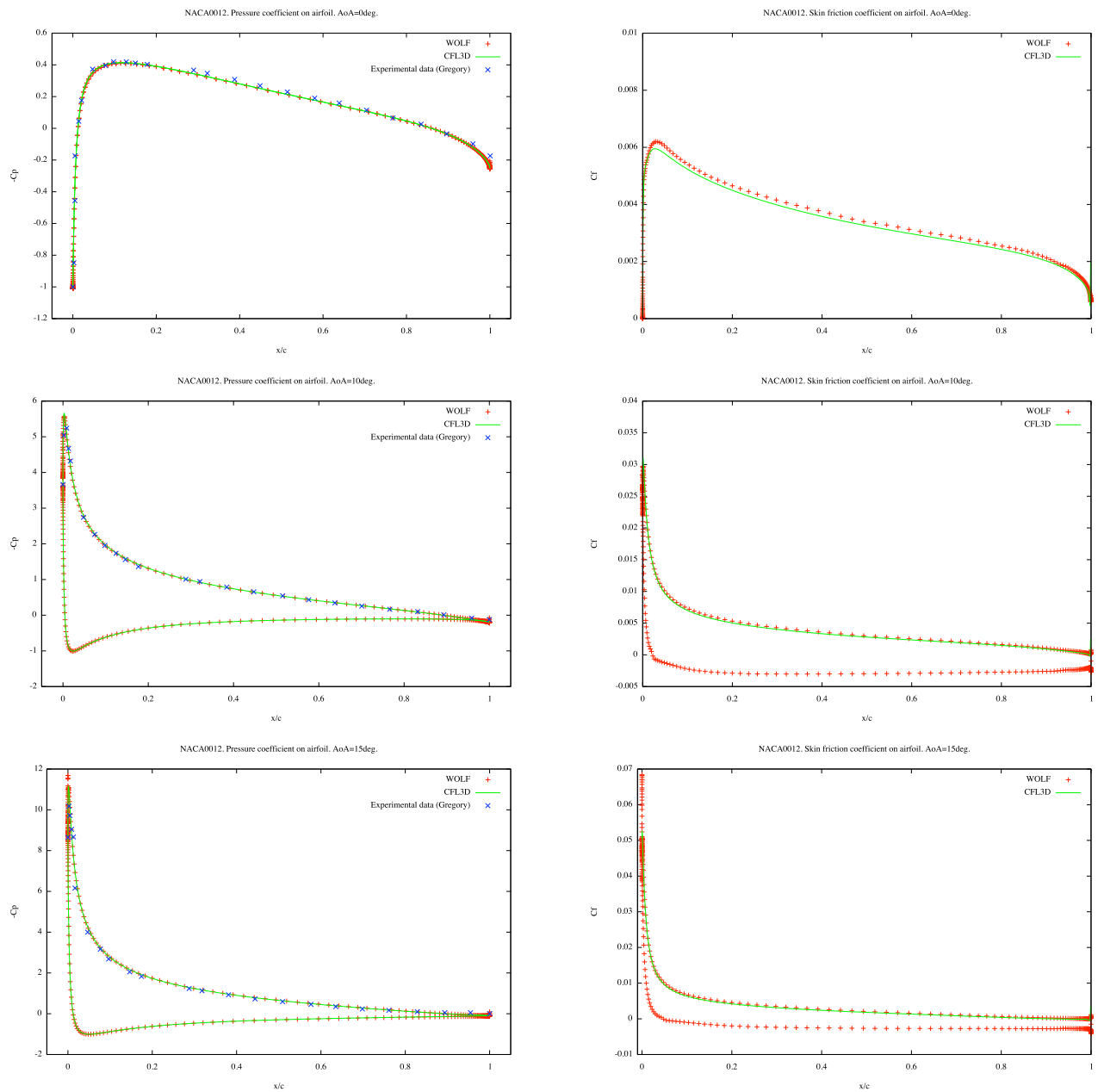
Figure 5. NACA0012: Pressure coefficient C_p and skin friction coefficient C_f for \alpha = 0, 10, 15 deg. Comparison with experimental data ( C_p ) and CFL3D ( C_p and C_f ).
