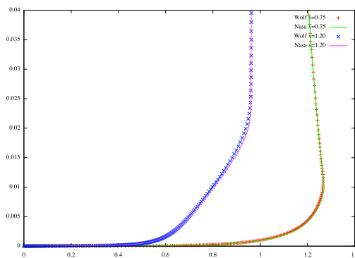
Figure 2. Bump: Velocity profiles
