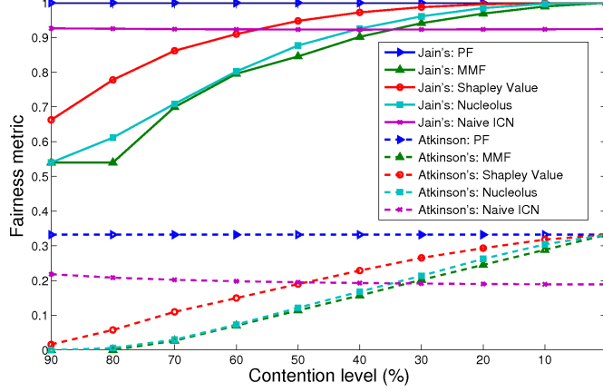
Figure 6: Fairness indexes as a function of the contention level (the lower the contention level, the higher the available cache size with respect to demands), for different allocation rules.
