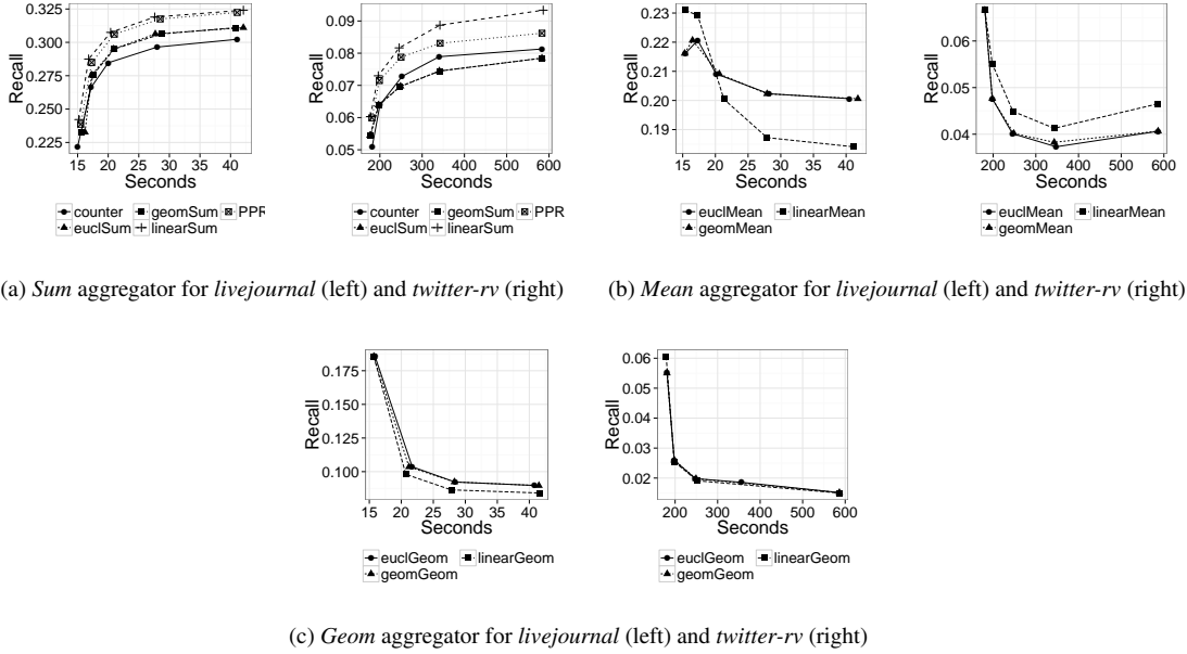
Figure 8: Comparison of computing time against recall for different scoring configuration. Each point corresponds to a different configuration with k_{local} = 5, 10, 20, 40, 80 running on 256 cores. The sum aggregator gets the highest recall, improving as k_{local} grows.
