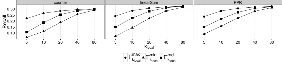
Figure 7: Recall obtained for three different neighbor sampling policies using k_{local} = 5, 10, 20, 40, 80 with the livejournal dataset. Selecting the most similar vertices ( \Gamma_{k_{local}}^{max} ) improves the recall, in particular for small values of k_{local} .
