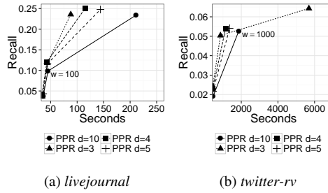
Figure 11: Recall and computing time using a stand-alone link-prediction solution on top of Cassovary using random walks to emulate PPR. Both solutions are run on a type-II machine with w = 10, 100, 1000 .
