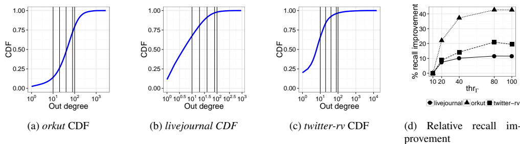
Figure 6: Relative recall improvement for different thr_\Gamma values when compared with the one obtained using thr_\Gamma = 10 with linear combinator. We highlight the used thr_\Gamma values in the CDF of the output degrees of the analyzed datasets. When thr_\Gamma reaches around 80% of the observations in the CDF there is no longer improvement.
