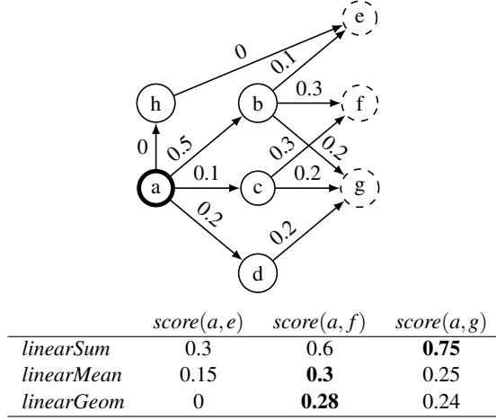
Figure 3: Example of scores obtained using different aggregators and the linear combinator with \alpha = 0.5 . Edge weights indicate the similarity between vertices.
