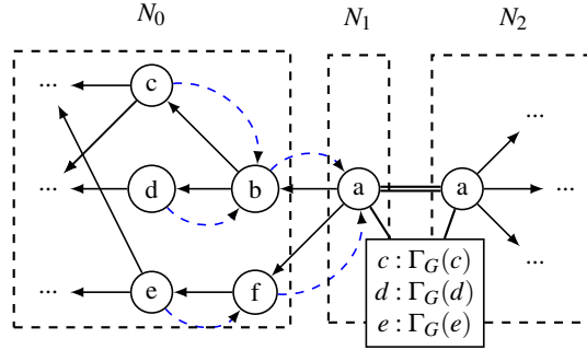
Figure 1: Example of data propagation in order to compute score(a,c) , score(a,d) and score(a,e) following a naive GAS approach for a graph deployed into three different computing nodes ( N_0 , N_1 and N_2 ). We have to propagate \Gamma_G(c) , \Gamma_G(d) and \Gamma_G(e) through b and f (dashed blue arrows). Then, this information has to be transferred to vertex a which is allocated into a different machine ( N_1 ). Additionally, this information has to be replicated onto the replicas of a for synchronization.
