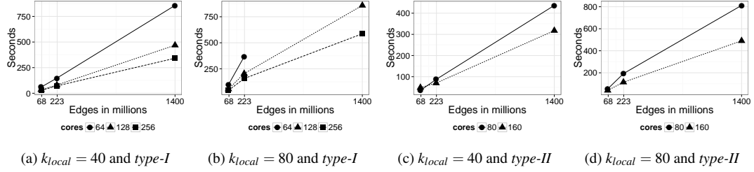
Figure 5: SNAPLE scales linearly graph sizes (measured in edges). Execution times are reported for both type-I and type-II nodes, and for k_{local} \in \{40, 80\} . Missing points indicate configurations not fitting into memory.
