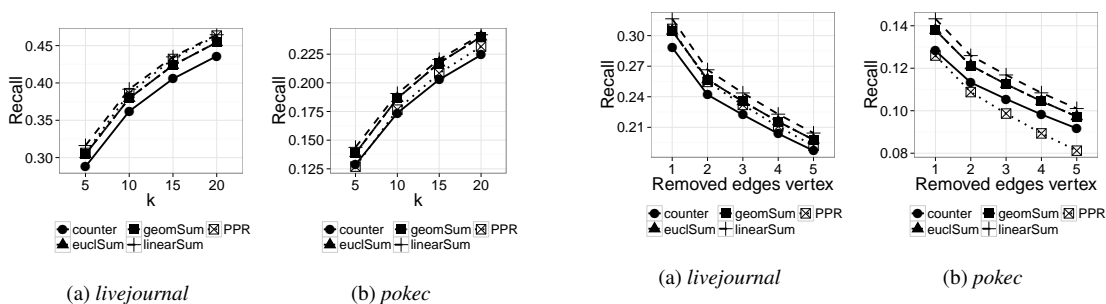
Figure 10: Evolution of recall when increasing the number of removed edges per vertex with k_{local} = 80 .
