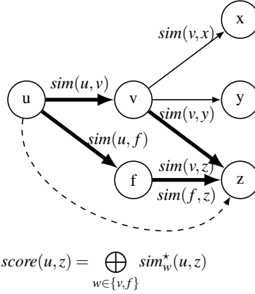
Figure 2: Two paths connect u to z , resp. through v and f . Each path yields different similarity values: sim_v^*(u,z) and sim_f^*(u,z) . To summarize these different values, SNAPLE aggregates them using an aggregator ( \oplus , Table 2).
