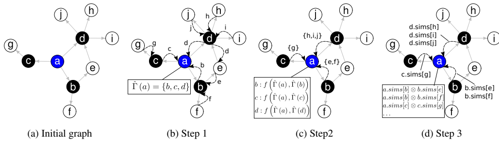
Figure 4: Illustrating Algorithm 2. In Step 1, each vertex constructs its list of neighbors \hat{\Gamma} . This list of neighbors is propagated to adjacent vertices (Step 2) to compute raw similarities sims[\cdot] (for a : with c , d , and b ). Only the k_{local} most similar vertices are kept. Finally (Step 3), raw similarities are used to compute path similarities, which are then combined into final scores.
