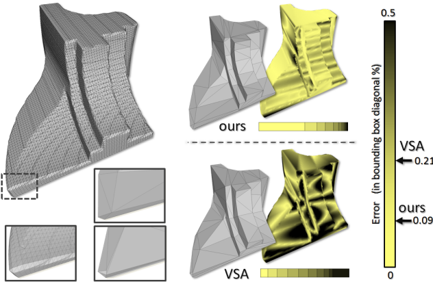
Figure 9: Comparison with VSA. A model of a Fandisk reconstructed with a voxel-based method (available from AIM@Shape repository) is decimated to 77 vertices with our method (top right) and VSA (bottom right). Our method yields a lower mean error than VSA.
