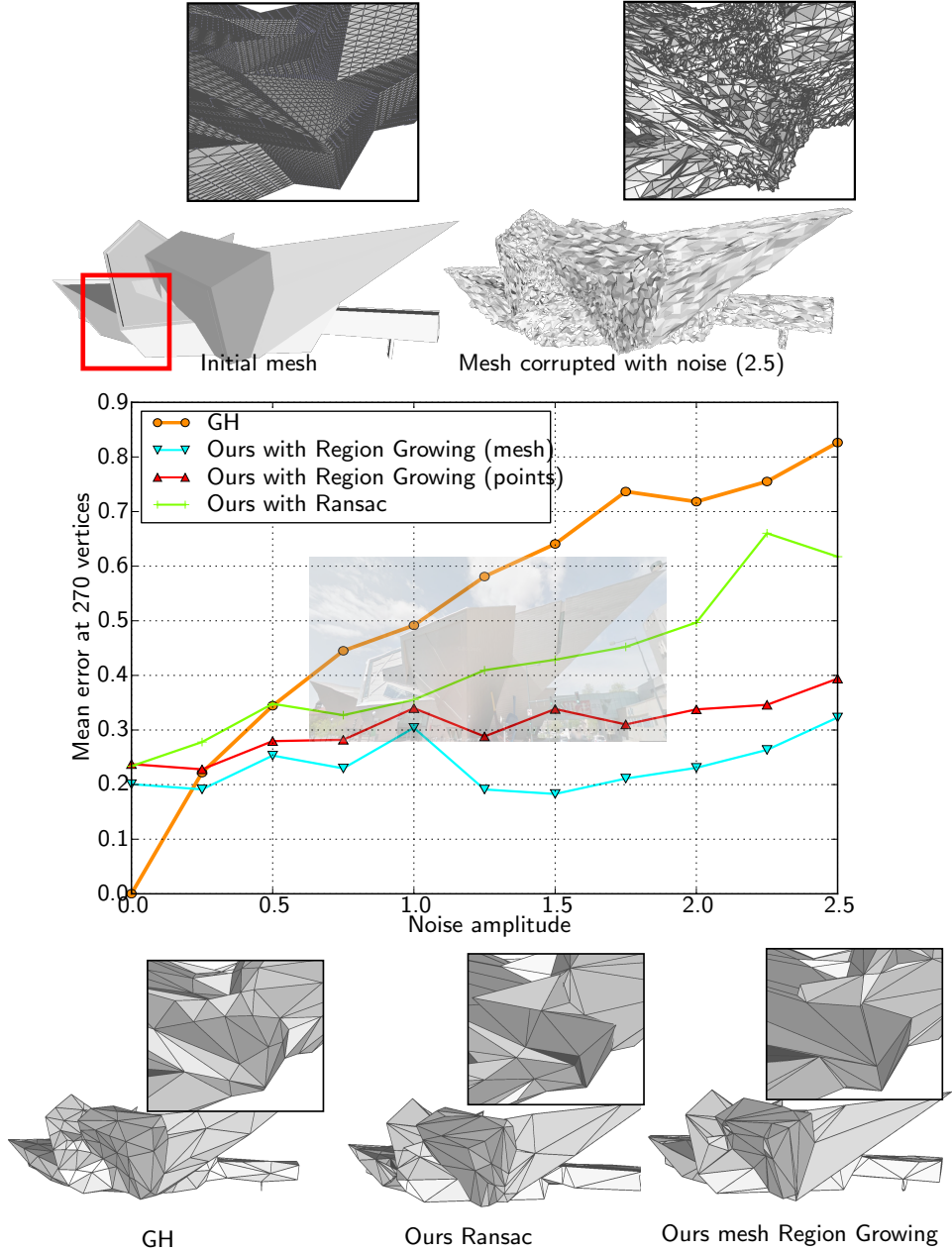
Figure 17: Noise robustness for three planar detection methods. A dense mesh of the Denver museum (upper left) is decimated after being corrupted by various levels of uniform noise. The curves plot the mean error against noise, measured after the input mesh model (40,000 vertices) is decimated to 270 vertices with Garland-Heckbert (GH) and our method. We combine our approach with (1) planar proxies detected via RANSAC, region-growing based on the mesh triangles and region-growing based on the mesh vertices (with a 10-nearest neighbors graph). The planar proxies are detected with the same parameters for all noise values. When the mesh is corrupted with noise, our algorithm with region growing yields a nearly uniform error in this range and lower than Garland-Heckbert. However, in absence of noise, our method generates an extra error mainly due to abstraction. RANSAC yields lower results than region-growing in this case, which is expected since this method is primarily designed to be outlier robust.
