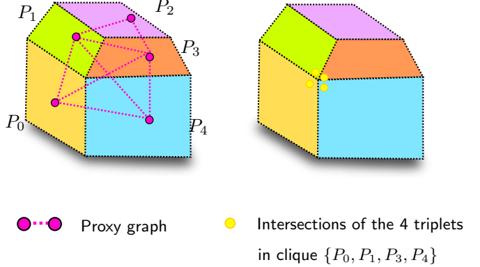
Figure 6: Multiple corners. The graph of proxies has a clique \sigma with size larger than 3. When the planes are not exactly aligned, intersecting all triplets included in \sigma yields \binom{|\sigma|}{3} distinct points.
