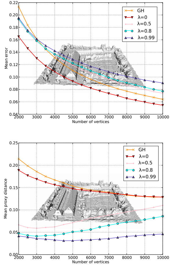
Figure 16: Complexity-distortion. We plot the mean error between the initial and approximated mesh (top) and the mean proxy distance (bottom) while decimating the mesh depicted by Figure 15, with four distinct values for the abstraction parameter \lambda . The mean proxy distance is computed as the average distance from vertices to their associated proxy. Higher values for \lambda yield lower proxy error but higher error for the approximation compared to the original mesh.
