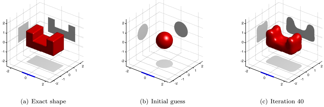
Figure 3: Reconstruction with \delta_0 = 2\% of noise and for four incident waves : \hat{\theta}_1 = -\hat{\theta}_2 = (0, 0, 1) , \hat{\theta}_3 = -\hat{\theta}_4 = (0, 1, 0) , \mathbf{p}_1 = \mathbf{p}_2 = (0, 1, 0) and \mathbf{p}_3 = \mathbf{p}_4 = (1, 0, 0) . The impedance parameters are \lambda = -0.25i and \eta = 0.25i .
