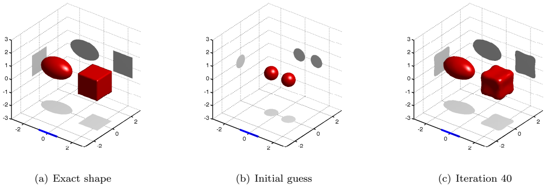
Figure 4: Reconstruction with \delta_0 = 2\% of noise and for four incident waves : \hat{\theta}_1 = -\hat{\theta}_2 = (0, 0, 1) , \hat{\theta}_3 = -\hat{\theta}_4 = (0, 1, 0) , \mathbf{p}_1 = \mathbf{p}_2 = (0, 1, 0) and \mathbf{p}_3 = \mathbf{p}_4 = (1, 0, 0) . The impedance parameters are \lambda = -0.25i and \eta = 0.25i .
