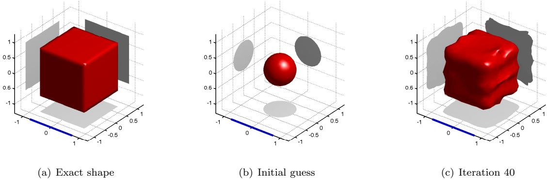
Figure 2: Reconstruction with \delta_0 = 2\% of noise and for two incident waves : \hat{\theta}_1 = -\hat{\theta}_2 = (0, 0, 1) and \mathbf{p}_1 = \mathbf{p}_2 = (0, 1, 0) . The impedance parameters are \lambda = 0.5 and \eta = 0 .
