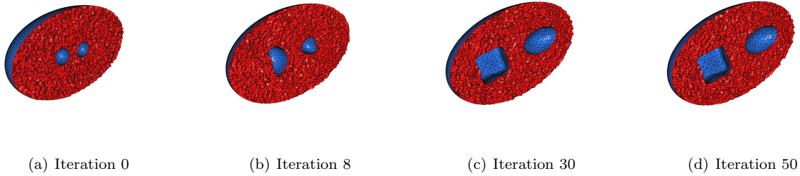
Figure 1: Different meshes obtained during the minimization procedure corresponding to Figure 4.
