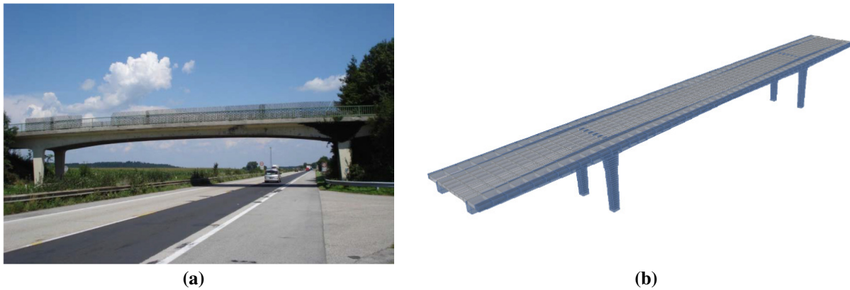
Fig 1 a S101 bridge structure, Austria, and b its calibrated finite element model
