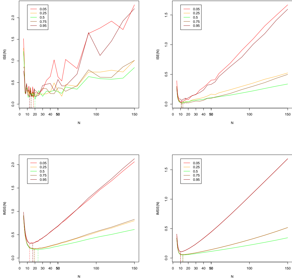
Figure 2: Plots of the mappings N \mapsto \text{ISE}_{\alpha}^{\wedge}(N) (top left) and N \mapsto \text{ISE}_{\alpha, B}^{-}(N) with B = 50 (top right) for a random sample of size n = 300 from Model ( \mathcal{M}1 ). The bottom panels report the corresponding plots obtained by averaging these mappings over m = 500 mutually independent random samples (all mappings are actually only evaluated at N = 5, 6, 7, \dots, 29, 30, 35, 40, \dots, 150 ).
