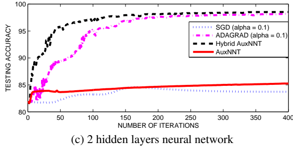
Fig. 2. Training and testing progress on MNIST database.
