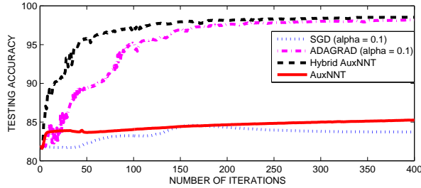
(c) 2 hidden layers neural network
