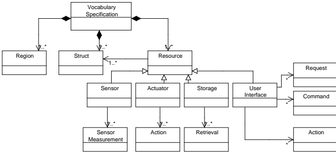
Figure 4 – Class diagram of domain-specific concepts
