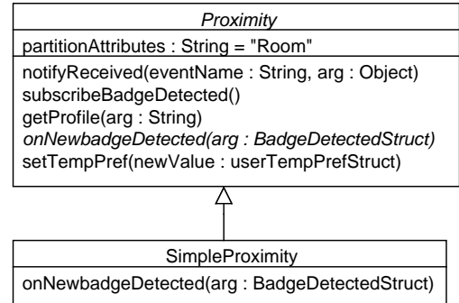
Figure 8 – Class diagram represents (1) the abstract class Proximity with its abstract method onNewbadgeDetected() illustrated in italicized text, and (2) the concrete implementation of onNewbadgeDetected() method is the SimpleProximity class.
