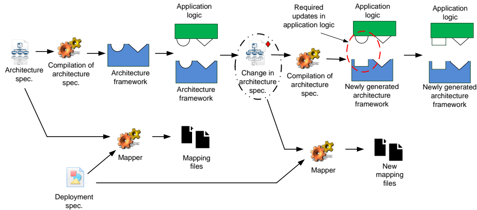
Figure 11 – Handling evolution in the functional concern
