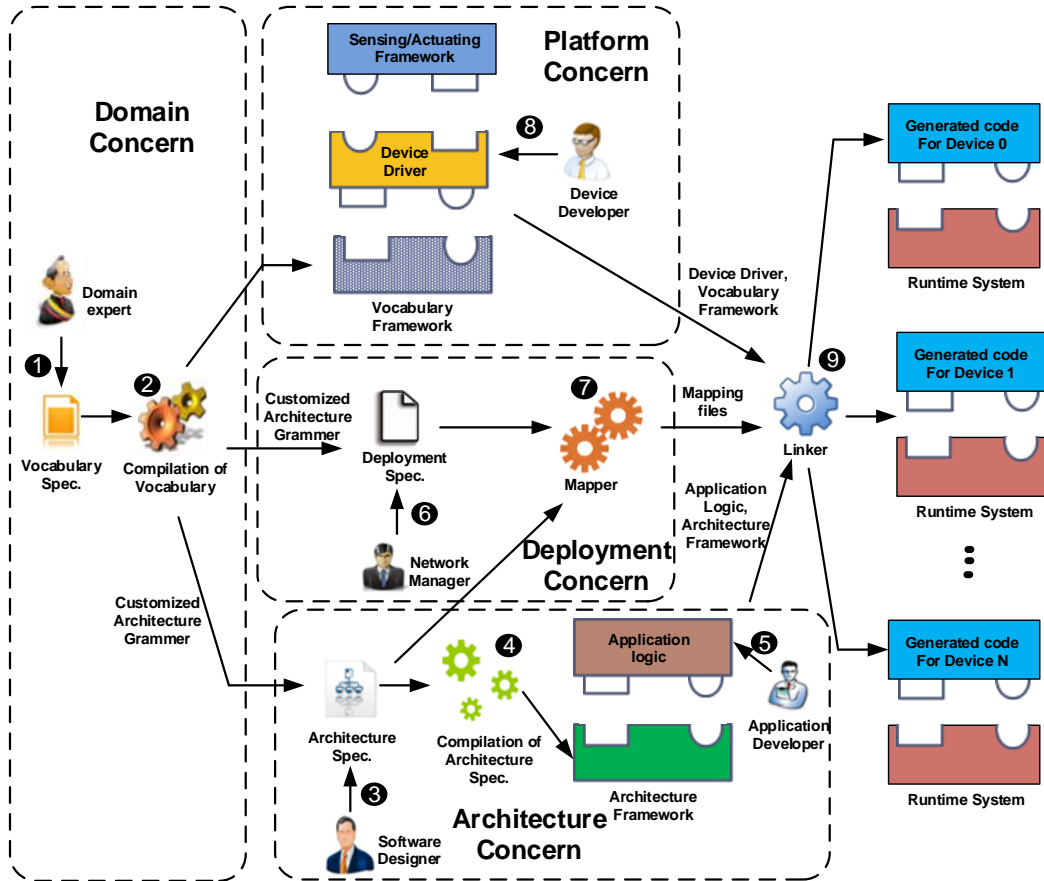
Figure 3 – IoT application development: overall process
