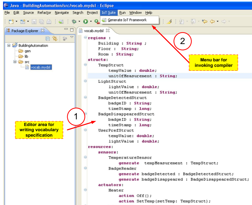
Figure 12 – Editor support for writing vocabulary specification in IoT Suite.
