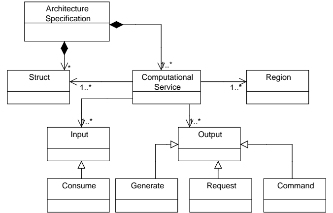
Figure 5 – Class diagram of functionality-specific concepts
