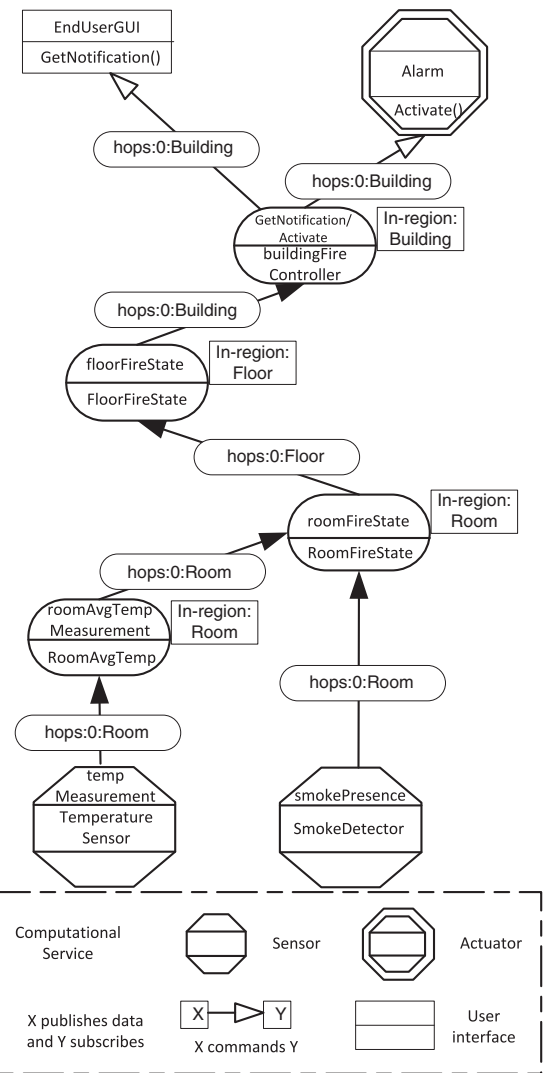
Fig. 15. Architecture of the fire detection application, similar to work in Cassou et al. (2011).
