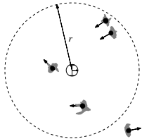
Fig. 1. Density features are computed by counting the number of human agents n contained in a circle of radius r and centered at the robot's position. In this example, the count is 4, corresponding to feature \phi_{d_2} .
