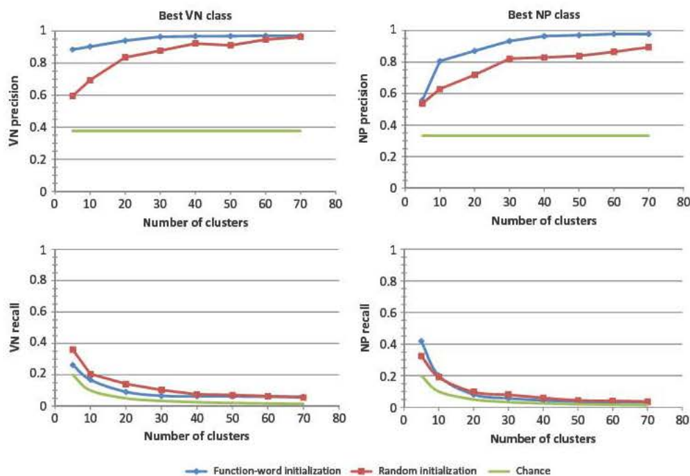
FIGURE 2 Precision and recall measures for the best VN and NP classes, as a function of the number of classes, in the different models. Standard error bars are not shown as they represent less than 0.1 points.
