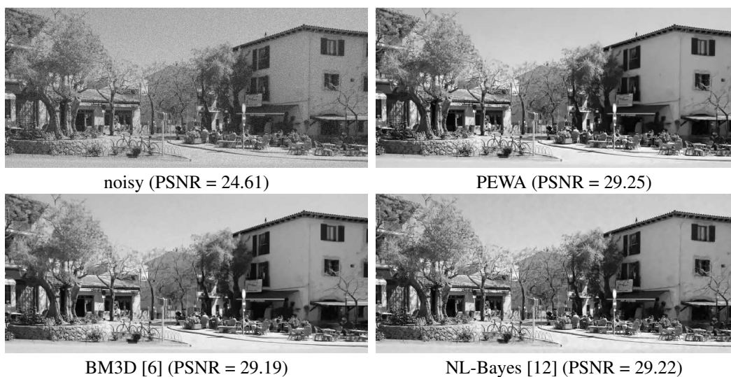
Figure 2: Comparison of algorithms. Valldemossa image corrupted with white Gaussian noise ( \sigma = 15 ). The PSNR values of the three images denoised with DCT-based transform [26] and combined with PEWA are 27.78, 27.04 and 26.26.
