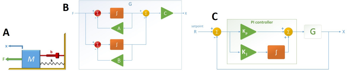
Figure 1: (A) Mass-spring-damper system. (Let F = 1 N, M = 1 kg, b = 10 N s/m, k = 20 N/m.) (B) MSD model, where triangular blocks denote gain functions with their corresponding weights, rectangular blocks denote integrators, and circle blocks denote mixers for summation and/or subtraction. (Let A = 2.764 , B = 7.236 and C = 0.2236 .) (C) PI-controlled MSD model, where G is the plant shown in (B). (Assume the values of K_P and K_I are given in Fig. 2 D.)
