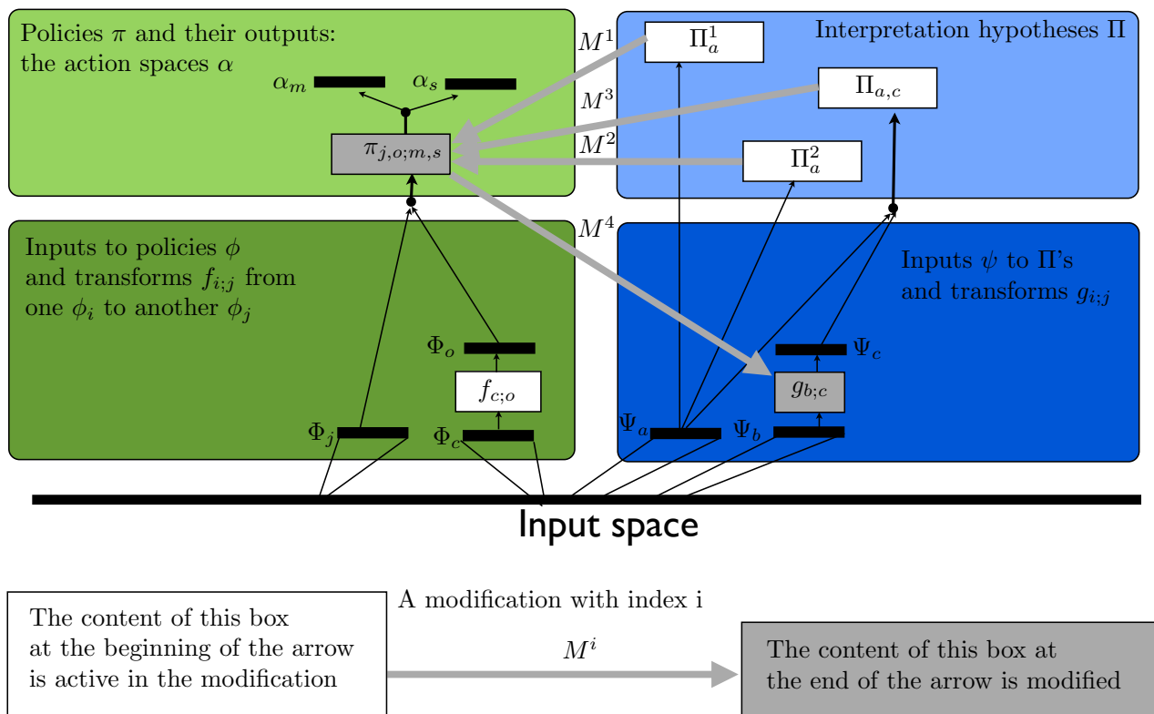
Fig. 1. In this setup, a policy \pi_{j,o;m,s} is modified by three interpretation hypotheses; \Pi_a^1 , \Pi_a^2 and \Pi_{a,c} . Inputs to policies are denoted \Phi and inputs to interpretation hypotheses are denoted \Psi . The black arrows mark inputs and the grey arrows mark modifications. The policy \pi_{j,o;m,s} is used to modify the transform g_{b;c} . If the policy \pi_{j,o;m,s} can be reasonably well learnt using only information in \Psi_a (for example a demonstration of a task), then it can later be used to check if the state in another space \Psi_c contains any useful information (for example, if one state is more frequent in the case where the demonstration was a failure, then this can be detected using \pi_{j,o;m,s} ). The informedness of states in a space \Psi_c can be judged using \pi_{j,o;m,s} (for example how useful states in \Psi_c are for separating failed demonstrations from successful ones). It is now possible to use \pi_{j,o;m,s} to choose from two different parameter settings of g_{b;c} (two different parameter sets result in two different \Psi_c spaces, which \pi_{j,o;m,s} can be used to choose between).
