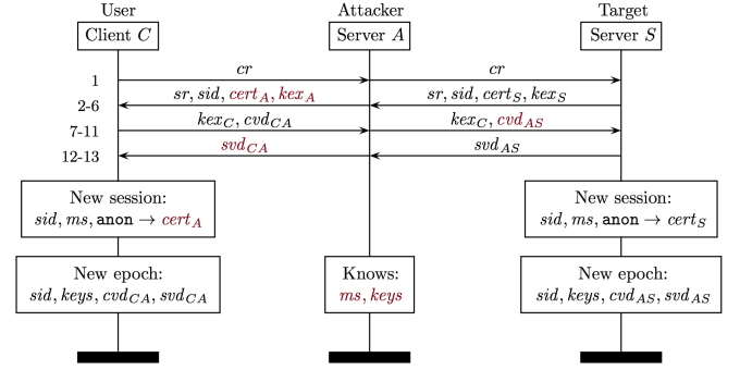
Connection 1: Full Handshake
