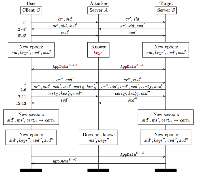
Connection 2: Session Resumption and Renegotiation
