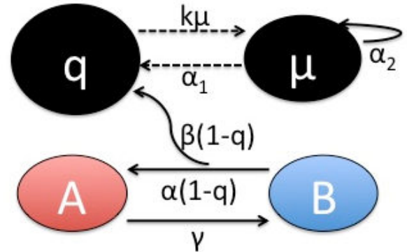
Fig. 3. Model conceptual scheme. Dashed and solid lines represent qualitative and quantitative relationships between variables, respectively
