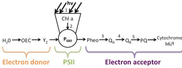
Fig. 1. Decomposition of the photochemical reaction steps. Chl a: chlorophyll a; P_{680} : reaction centre, Pheo: Pheophytin molecule; Q_A and Q_B : quinones A and B; PQ: plastoquinone; Y_z : a tyrosine molecule; OEC: Oxygen Evolving Complex; P: PSII; D and A: electron donors and acceptors.
