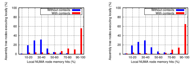
(a) Rucci1 on the MachineA platform using 40 cores.
