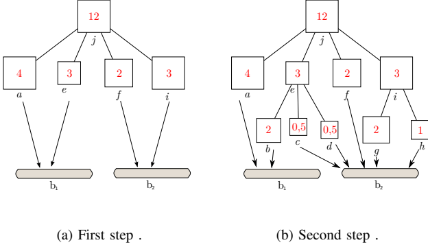
Fig. 2: Mapping algorithm.
