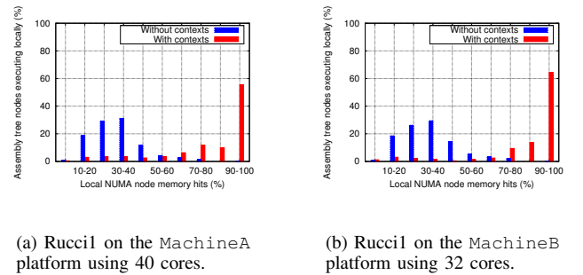
Fig. 6: Locality of data references for the Ruccl1 problem.
