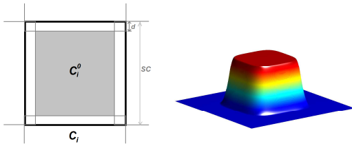
Fig. 9. Blending components in 2D: ( left ) The overlapping cells used to subdivide the domain; C_i^o shows the interior region; ( right ) the weighting function defined in (27) for blending IBS patches in 2D.
