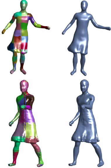
Fig. 8. Blended IBS: ( left ) different patch sizes ( N = 10, 20 ); ( right ) the blended surface using the proposed weighting technique.
