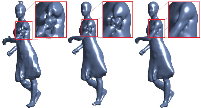
Fig. 17. Blended-IBS surface reconstruction is a good trade-off between local and global fitting: (left) MPU reconstruction ( \alpha = .75 ); (middle) RBF reconstruction; (right) Blended IBS surface reconstruction.
