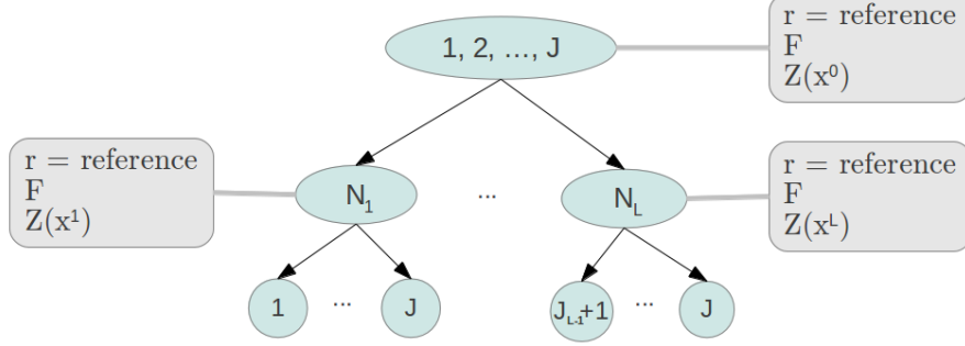
Figure 3: PCGLM for qualitative choices.
