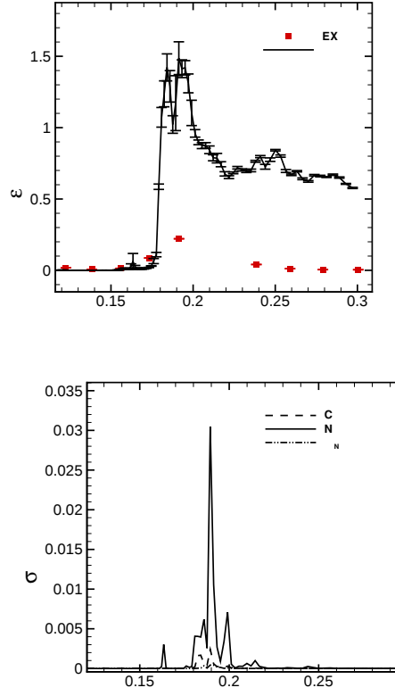
Figure 7: RMS wall pressure fluctuations along the profile, comparison between experimental data and numerical solutions (on the left), ANOVA analysis (on the right).
