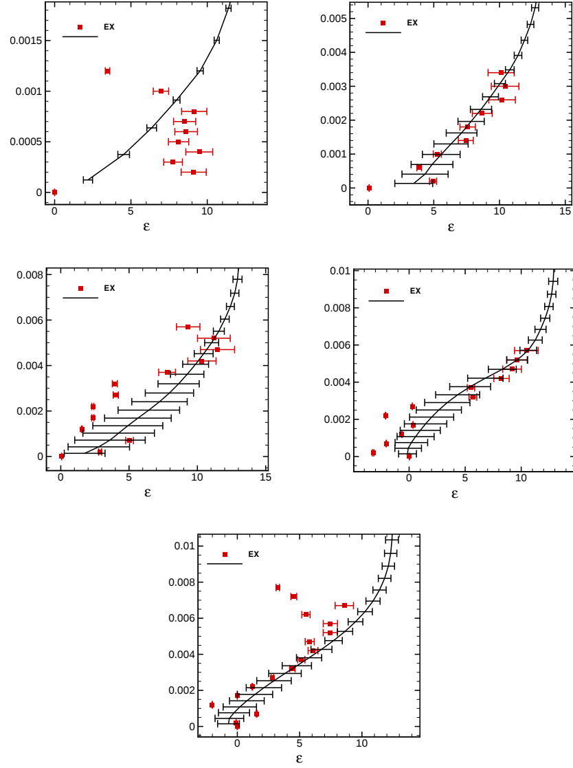
Figure 10: Comparison of numerical and experimental error bars for the velocity at the different stations described in Section 3.
