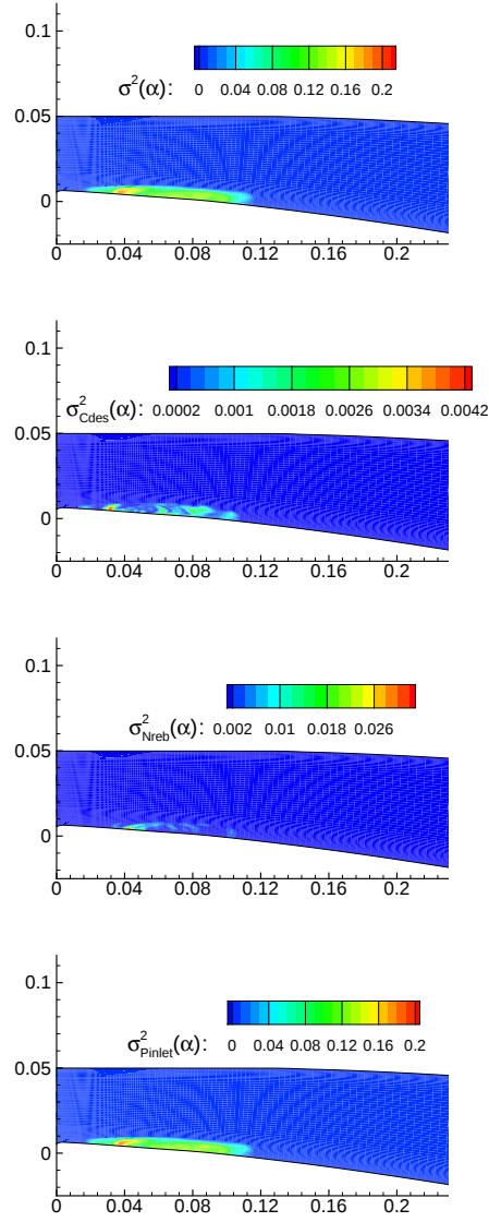
Figure 5: Sensitivity indices of the void ration at a time t = 1.5 s.
