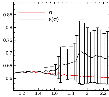
Figure 8: \sigma_{cav} along the profile.
