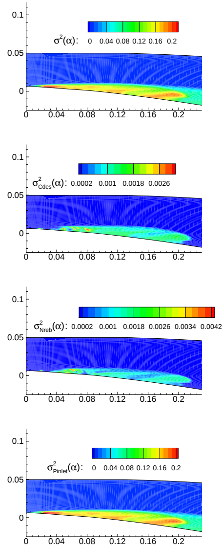
Figure 6: Sensitivity indices of the void ration at a time t = 2.28 s.
