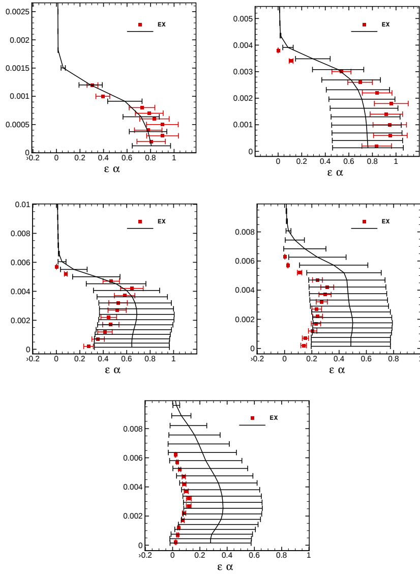
Figure 9: Comparison of numerical and experimental error bars for \alpha at the different stations described in Section 3.
