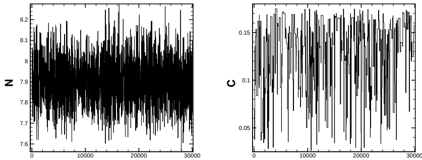
Figure 13: MCMC chain over 30,000 iterations, plotted in two dimensions for N_{reb} and C_{des} , respectively.
