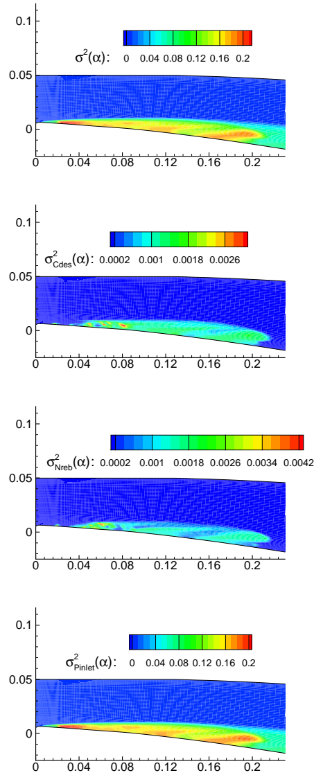
Figure 6: Sensitivity indices of the void ratio at a time t = 2.28 s.
