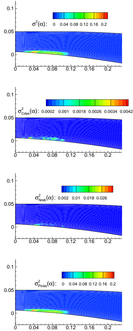
Figure 5: Sensitivity indices of the void ratio at a time t = 1.5 s.
